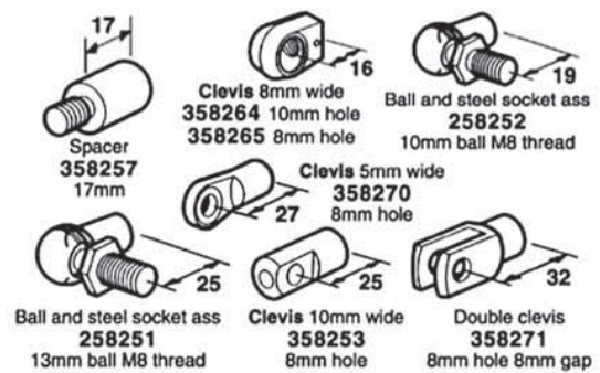
4100 Series 8mm End Fittings*
