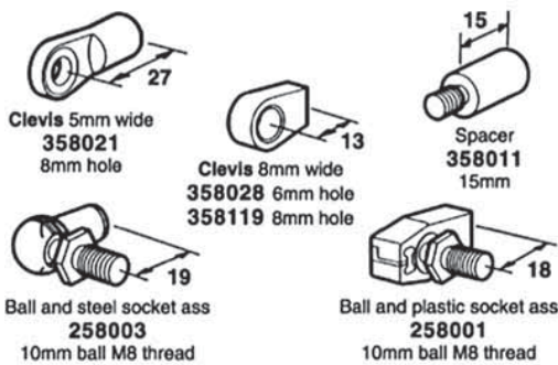
4000 Series 6mm End Fittings*
