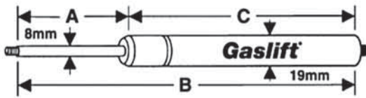
4000 Series 6mm End Fittings*
