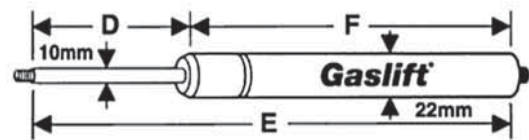
4100 Series 8mm End Fittings*
